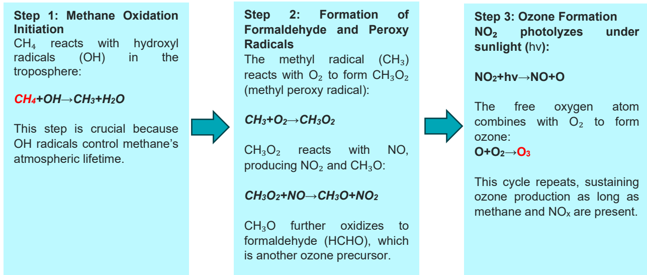
Figure 2-4 Methane role in O 3 formation
